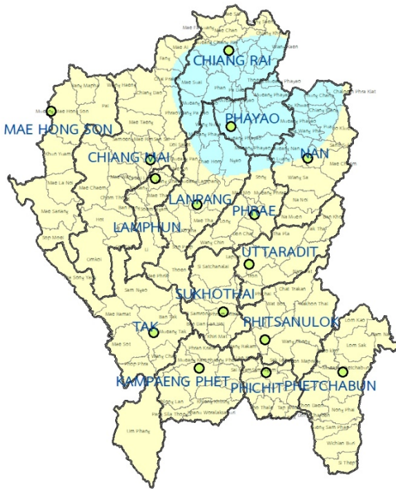
Minimum temperature forecast map
