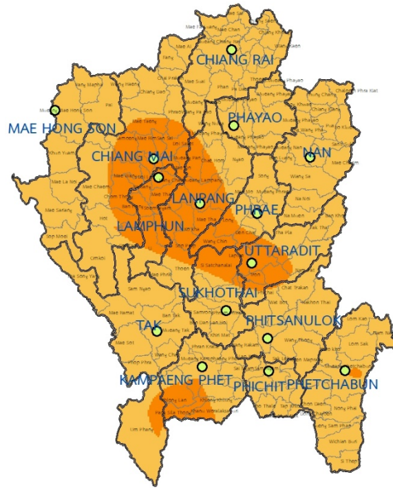
Maximum temperature forecast map
